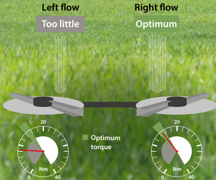
Classical weighing spreader
